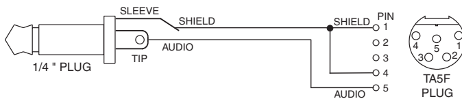
Wiring diagram
