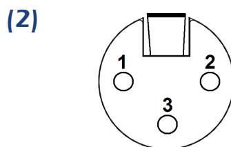
3-pin XLR female (solder side)
