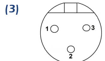
TA3F (solder side)
