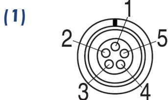
FGG.OB.305 (solder side)
